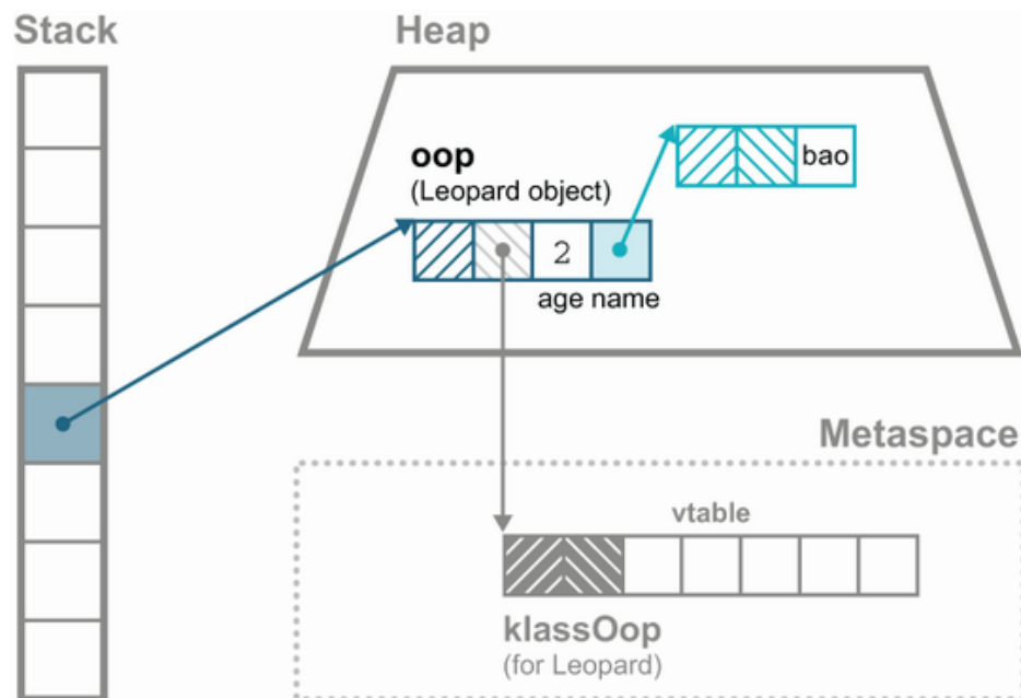
Figure 17.3 Locating a method implementation
