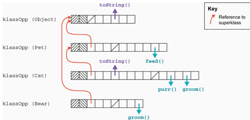
Figure 17.4 Vtable structure
