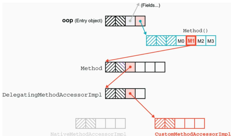
Figure 17.6 Implementing reflection
