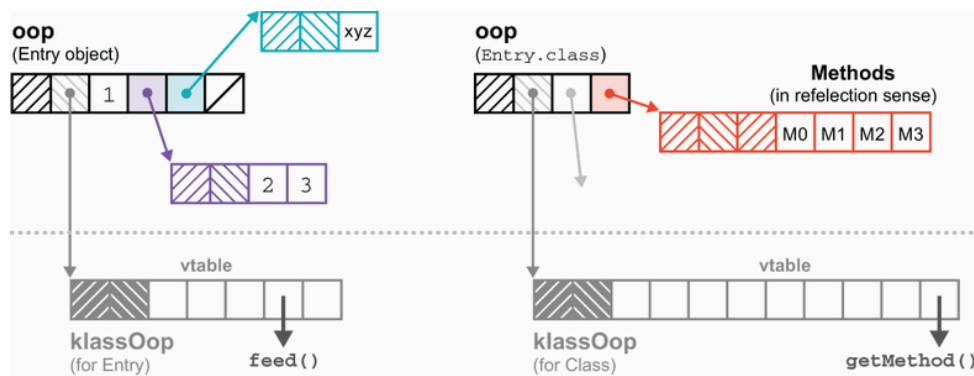
Figure 17.5 Reflection internals
