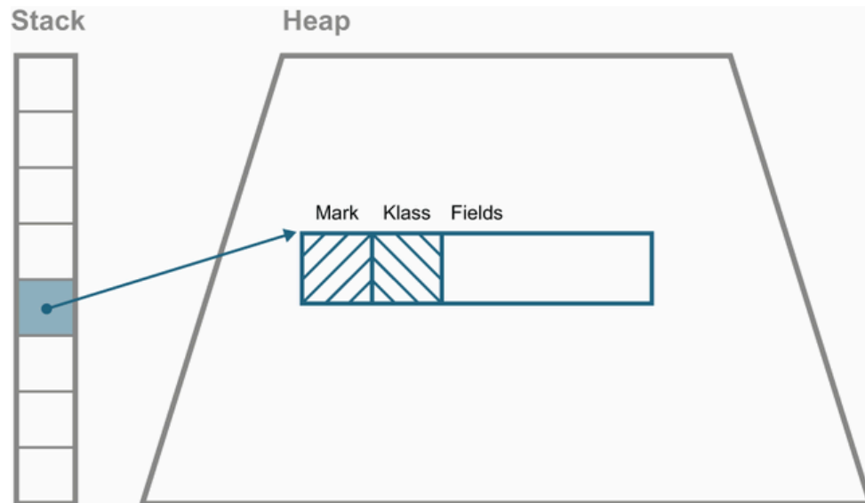
Figure 17.2 Java object header and layout
