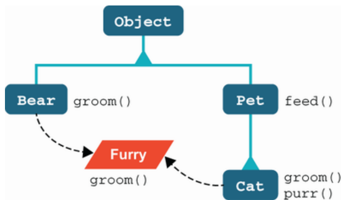
Figure 17.1 Simple inheritance hierarchy
